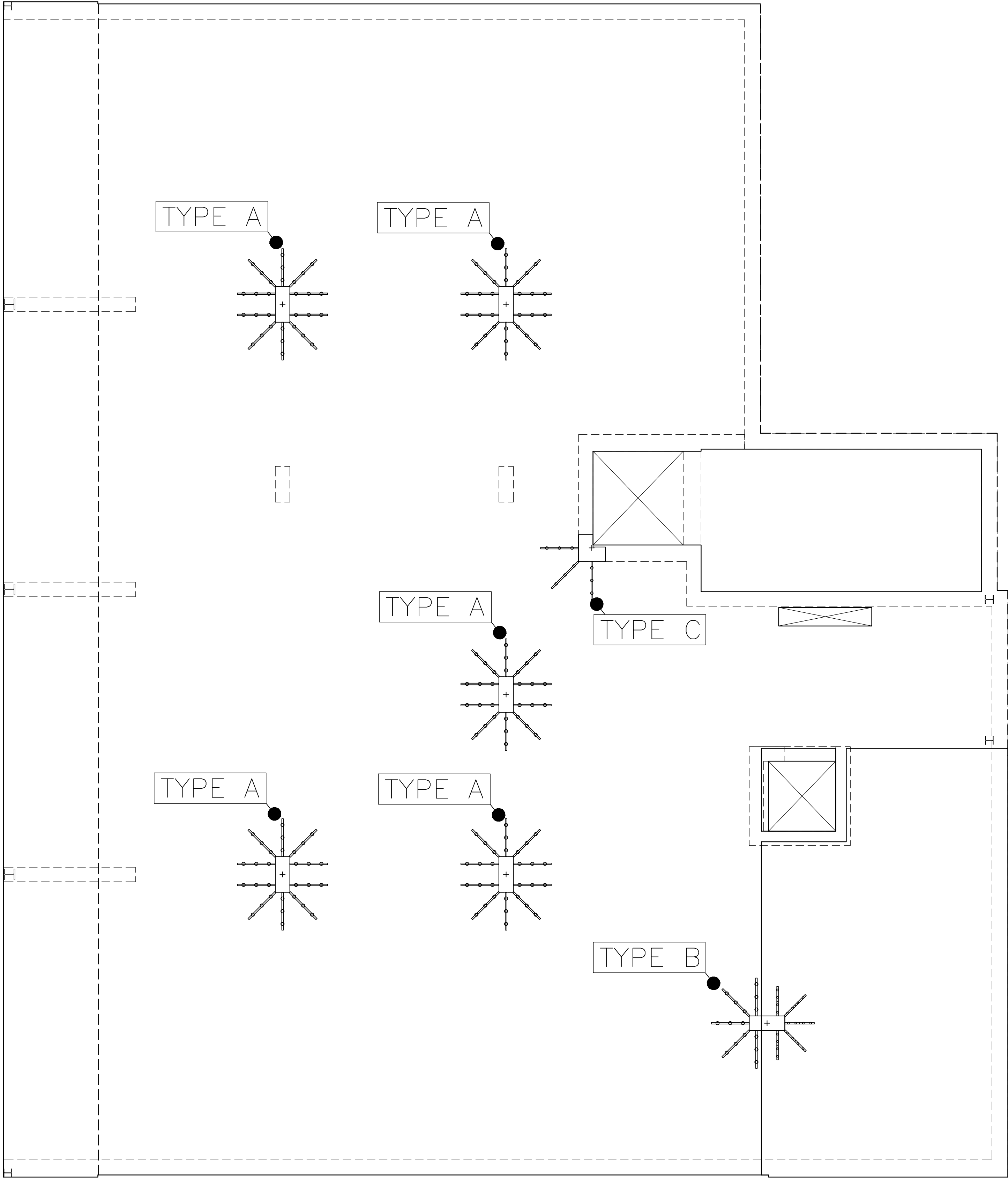
SHEAR RAIL LOCATION SCALE 1:50 © A1 SIZE SHEET
